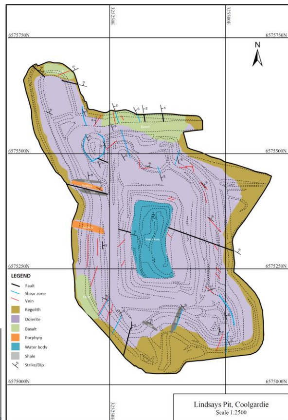
Figure 3 (Top). Geological map produced by traditional field mapping techniques.
